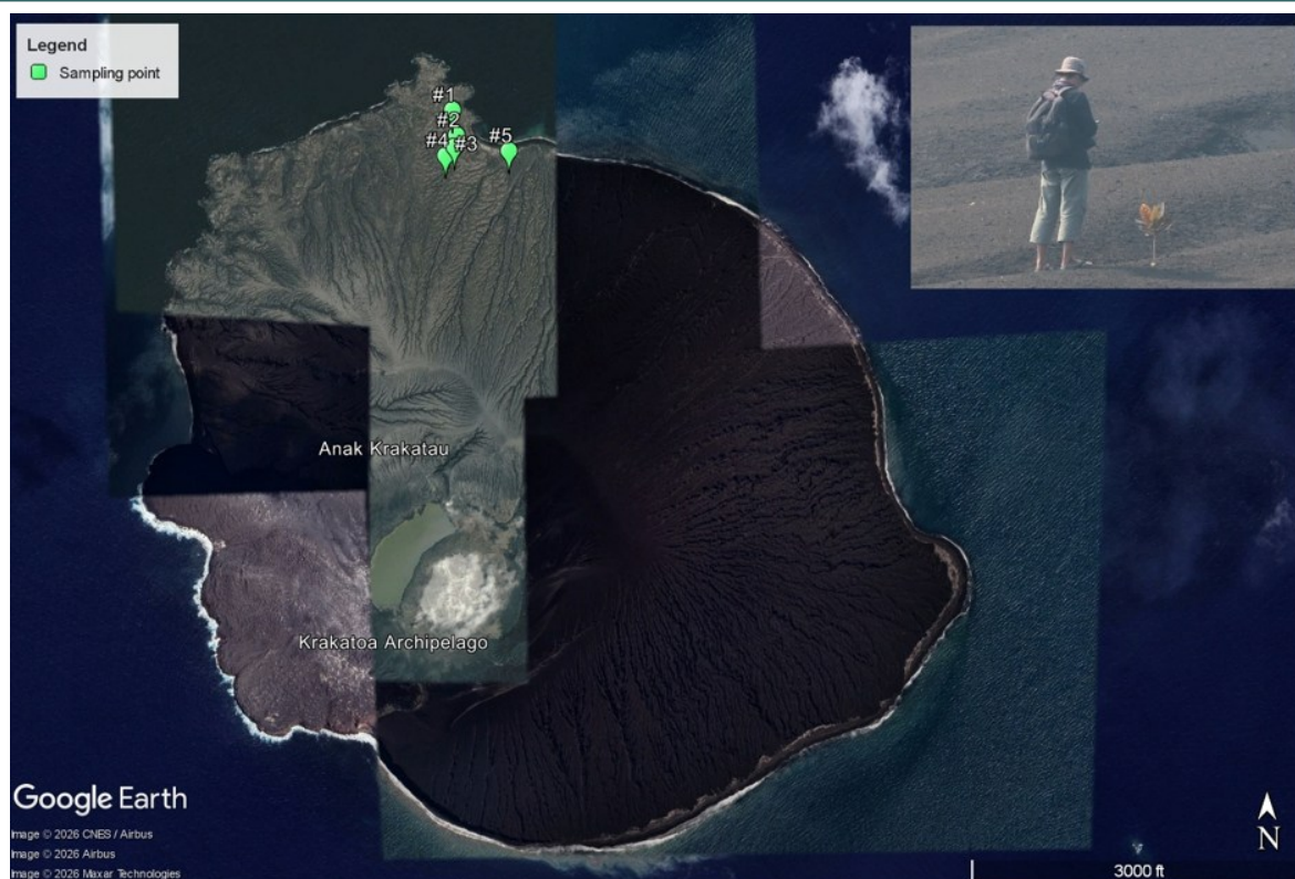
Figure 1. Location of soil sampling at Mount Anak Krakatau
